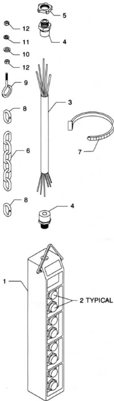
PUSHBUTTON STATION
