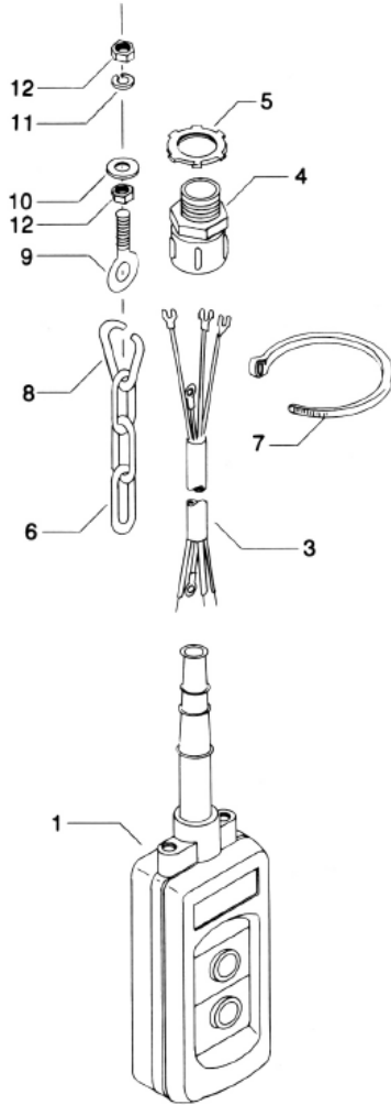
PUSHBUTTON STATION
