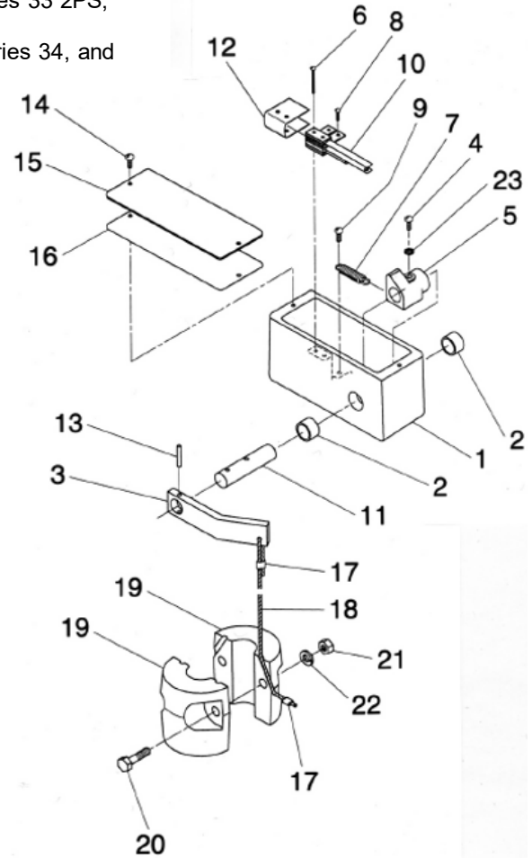
ASSEMBLY-01
