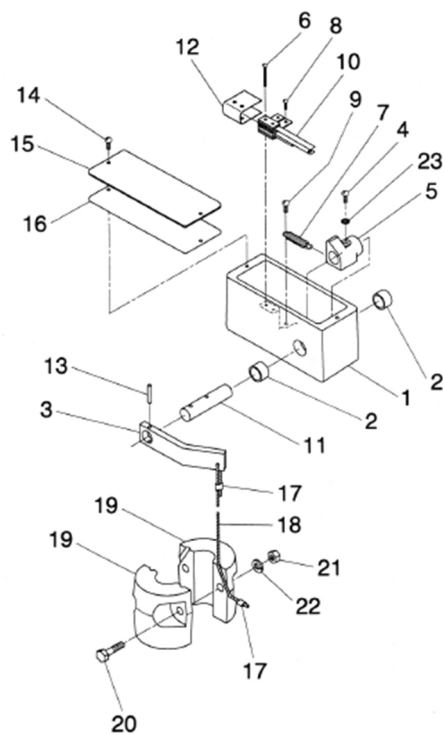
ASSEMBLY-01
