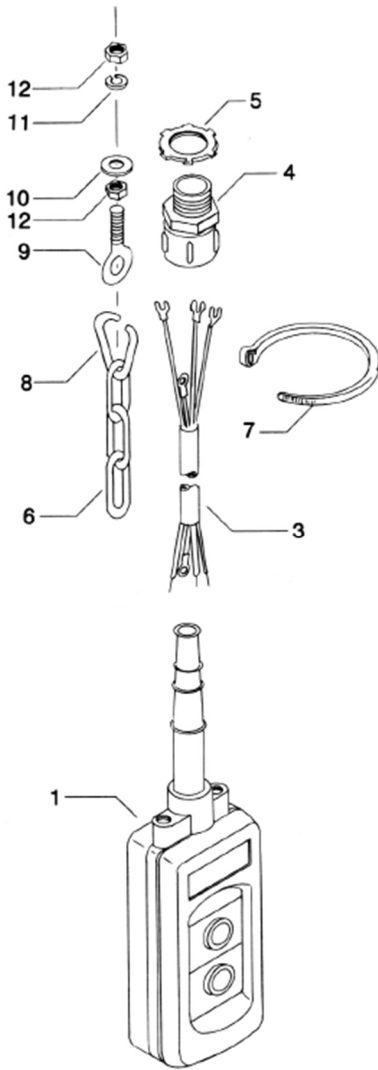
PUSHBUTTON STATION
