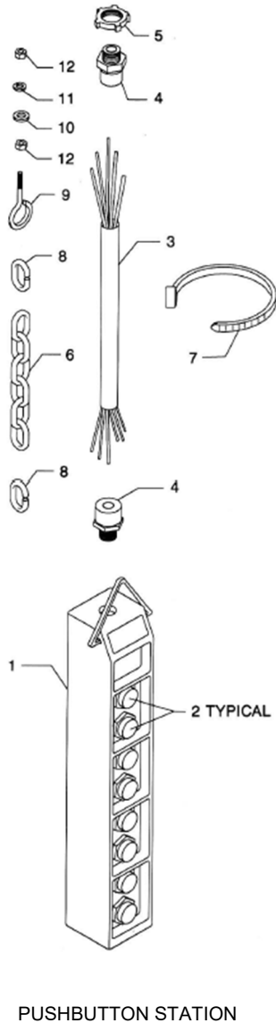
PUSHBUTTON STATION
