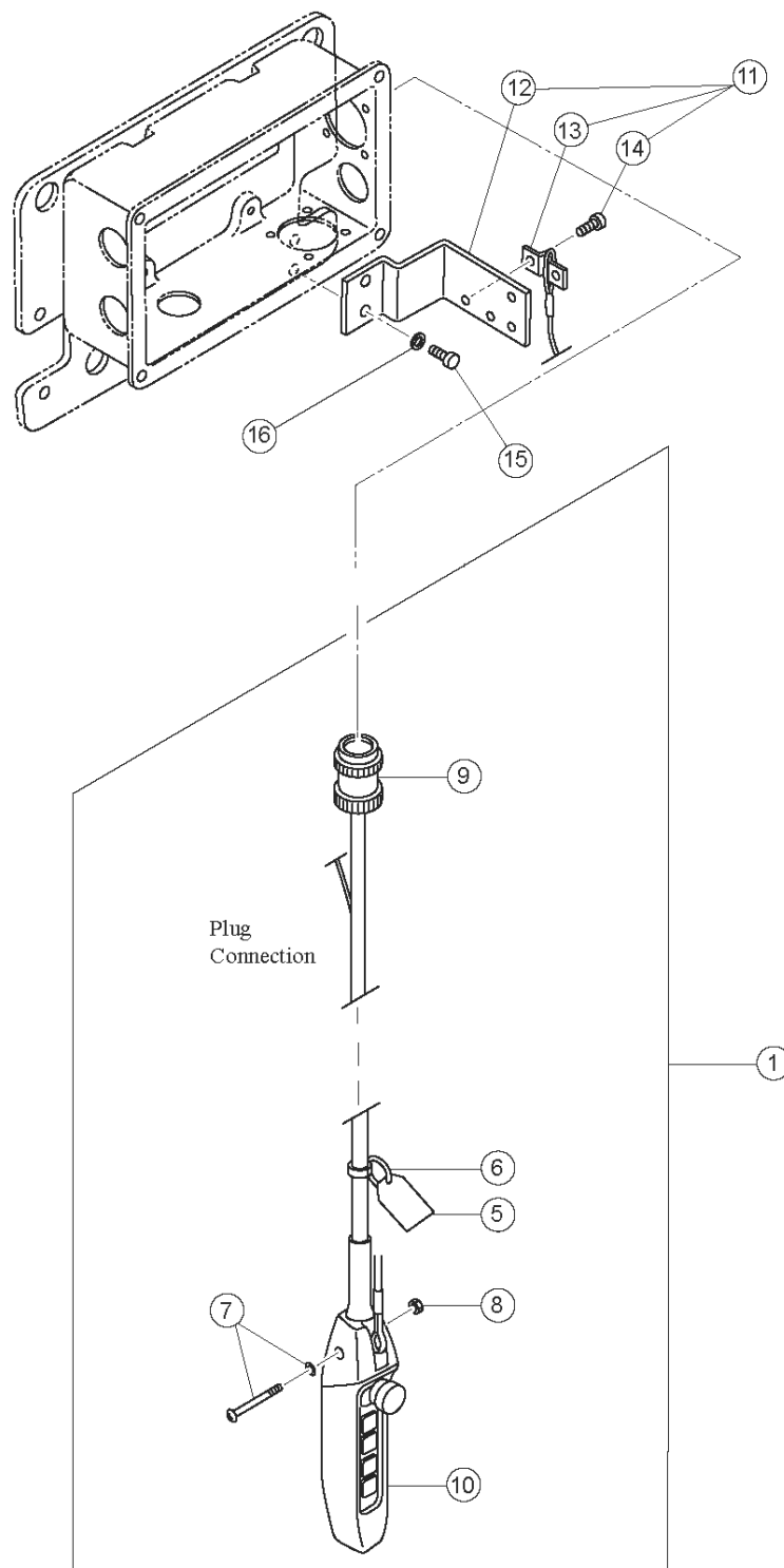
Figure 2-1 Pendant Parts
