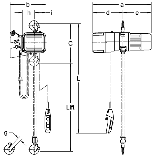
Figure 2-2 Dual Speed Hoist Dimensions
