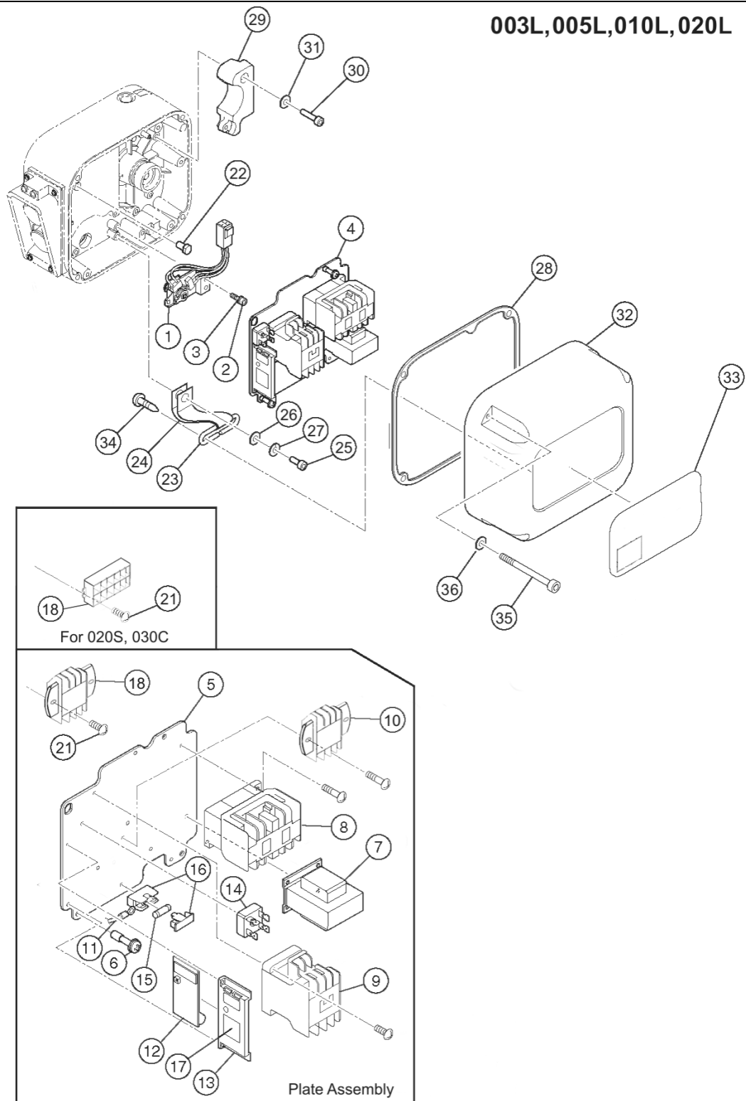
Figure 4-1 Electric Parts (Single Speed)
